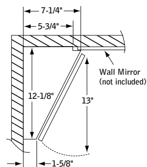
Top-down view of left hand Avanti 631 Corner Cabinet as shown in photo above.
