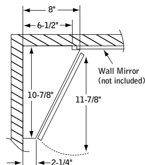
Top-down view of left hand Avanti 637 Corner Cabinet.
